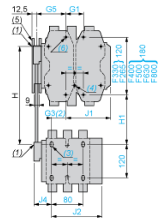
Assembly B (7) - Mechanical interlock reference
